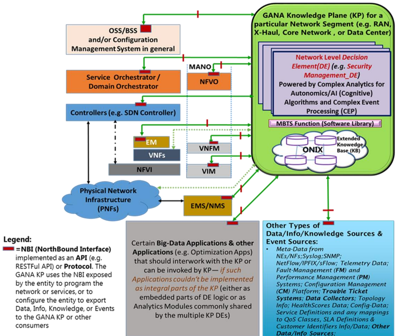
Figure 33: GANA KP's data sources diversity, events visibility and consumption into KP DEs; and KP Integration Options
