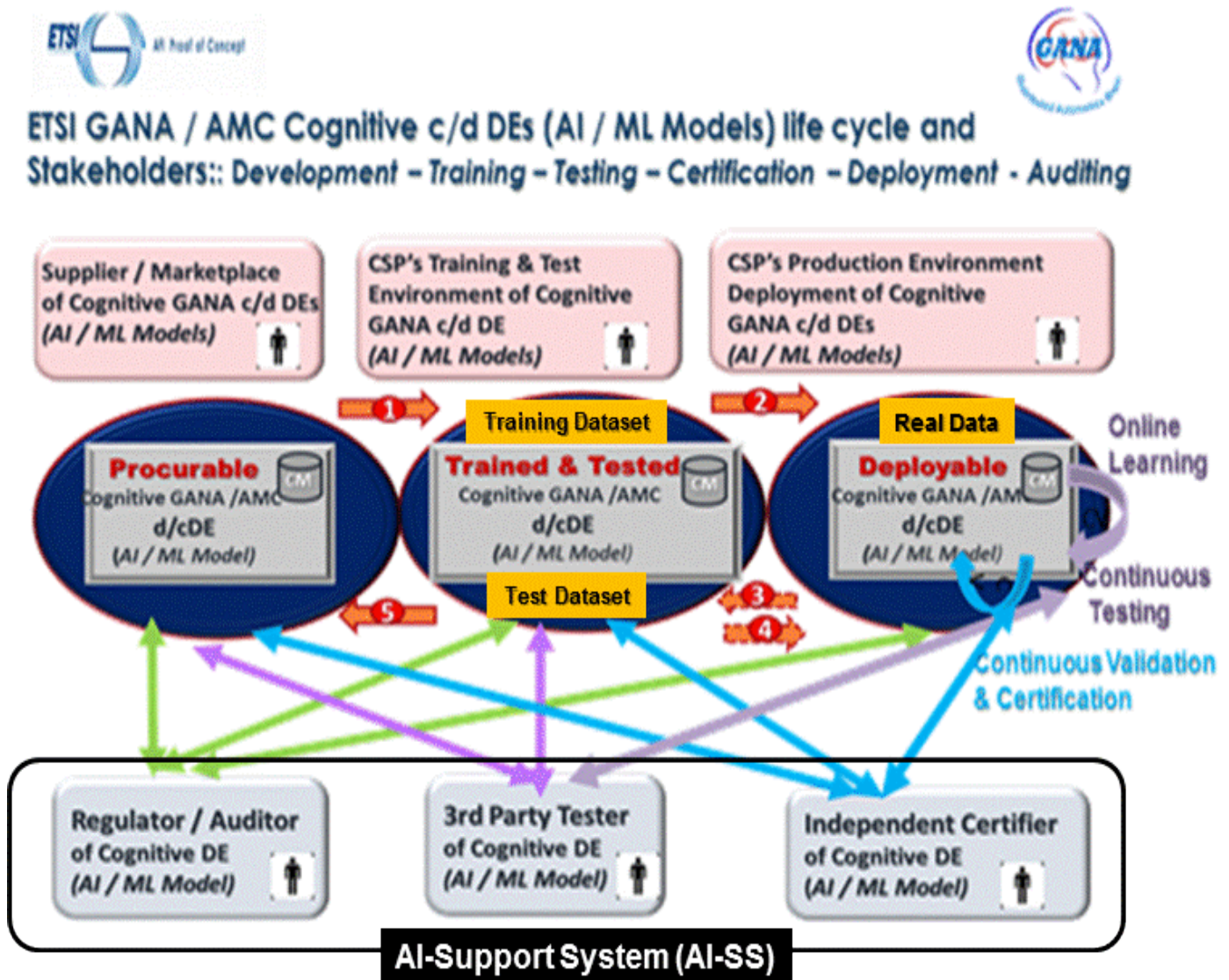
Figure 7: GANA AMC Cognitive c/d DEs (AI / ML Models) life cycle and Stakeholders: Development - Training - Testing - Certification - Deployment - Auditing (more details in White Paper No.4 [23])
